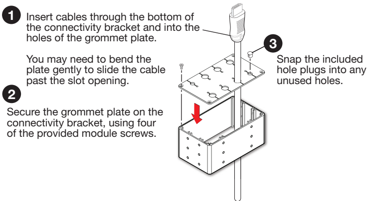
Figure 4. Assembling the Cable Pass-through Module
