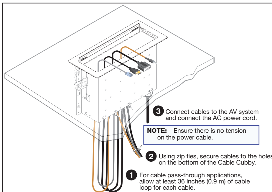
Figure 10. Route and Connect AV Cables
