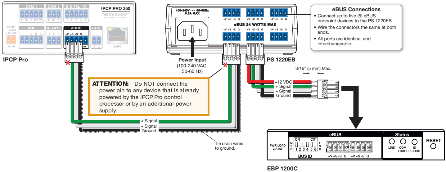
Figure 16. Powering an eBUS System with an PS 1220EB Power Inserter
