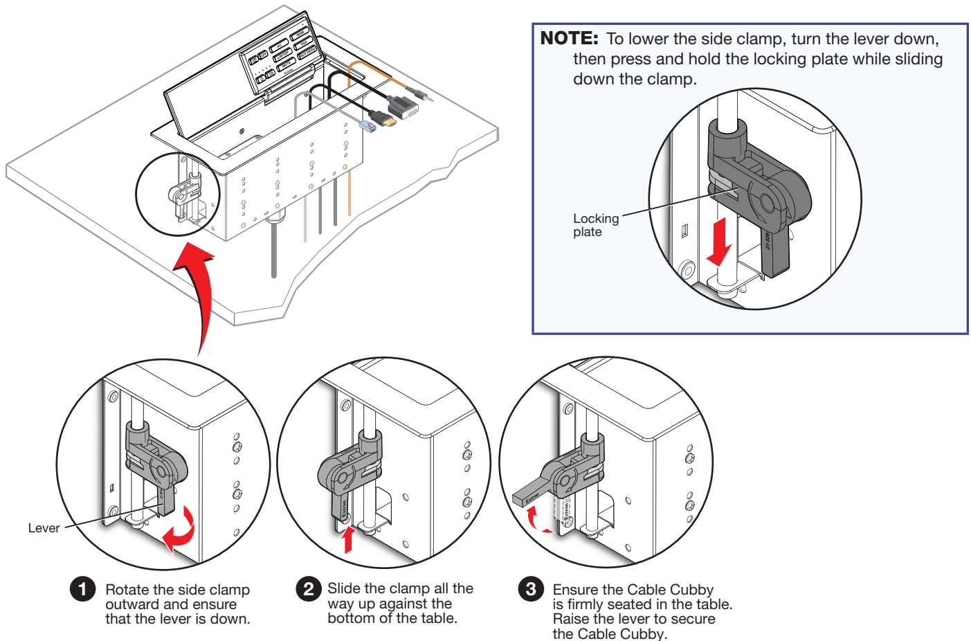
Figure 8. Secure the Cable Cubby Enclosure
