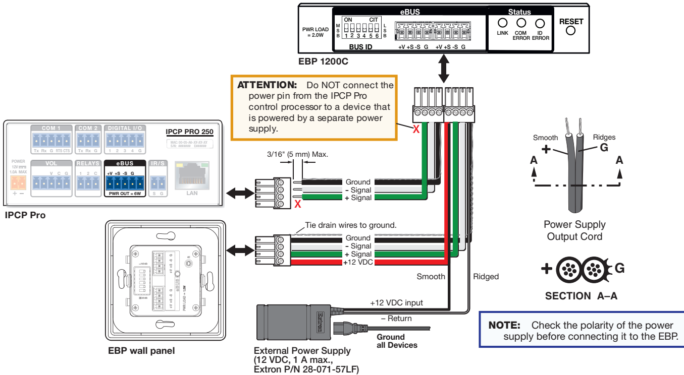
Figure 17. Powering an eBUS System with an Extron 12 VDC, 1A Power Supply
