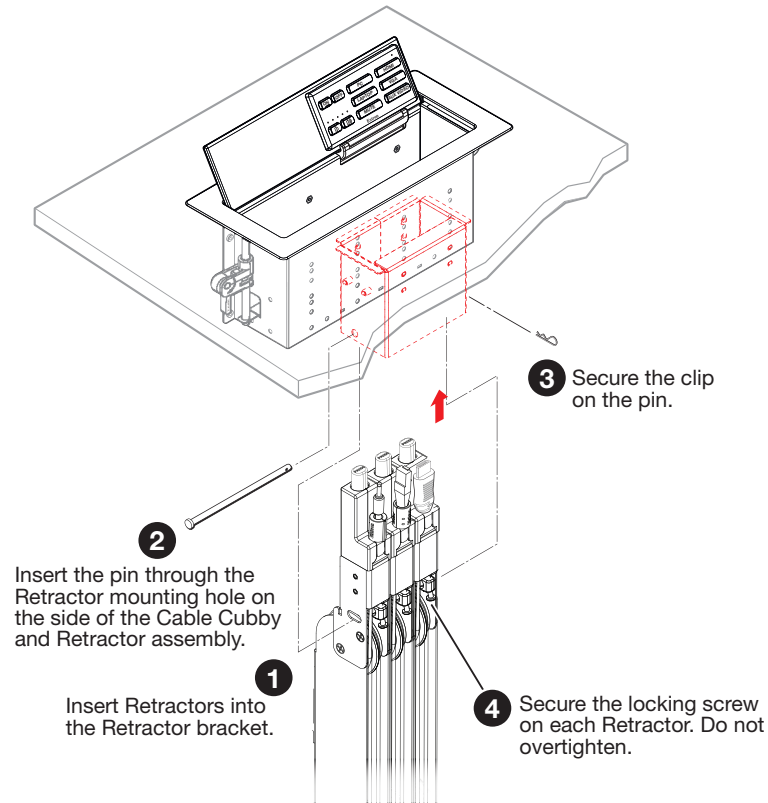
Figure 9. Installing Retractors
