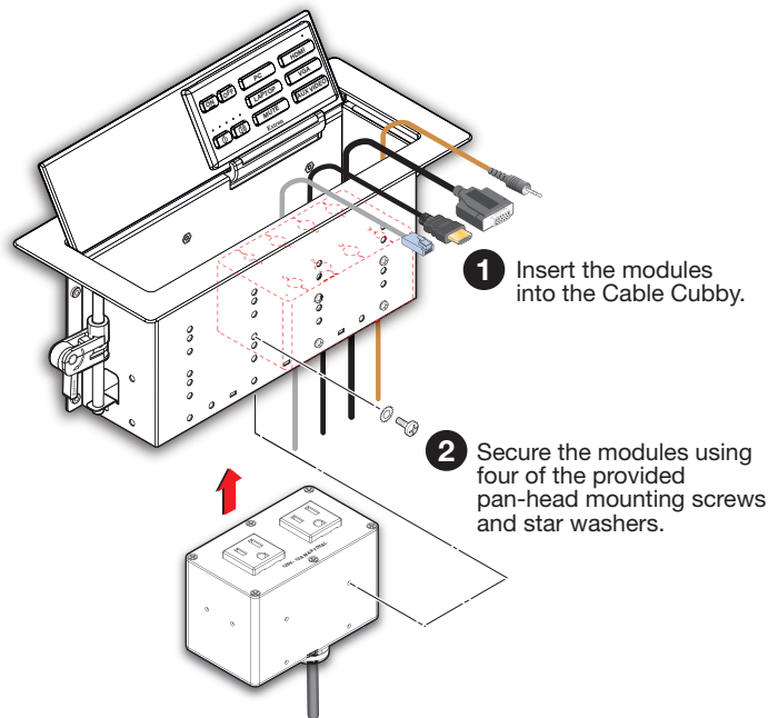
Figure 6. Install the Connectivity and Power Modules
