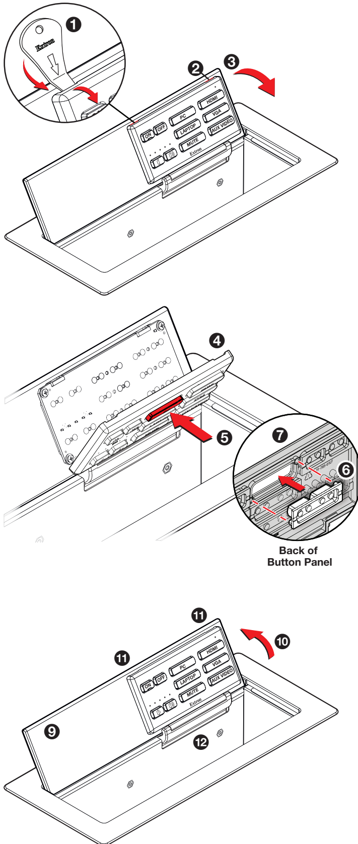
Figure 13. Replacing Buttons
