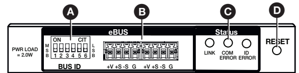
Figure 12. EBP 1200C Bottom Panel
