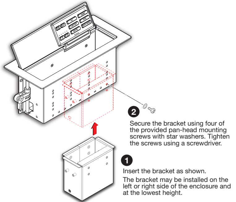
Figure 5. Install the Retractor Bracket
