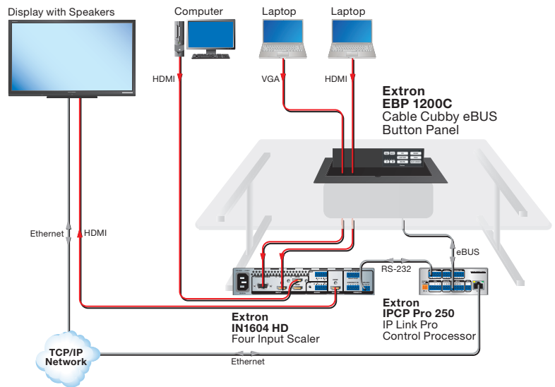
Figure 1. EBP 1200C Application Diagram
