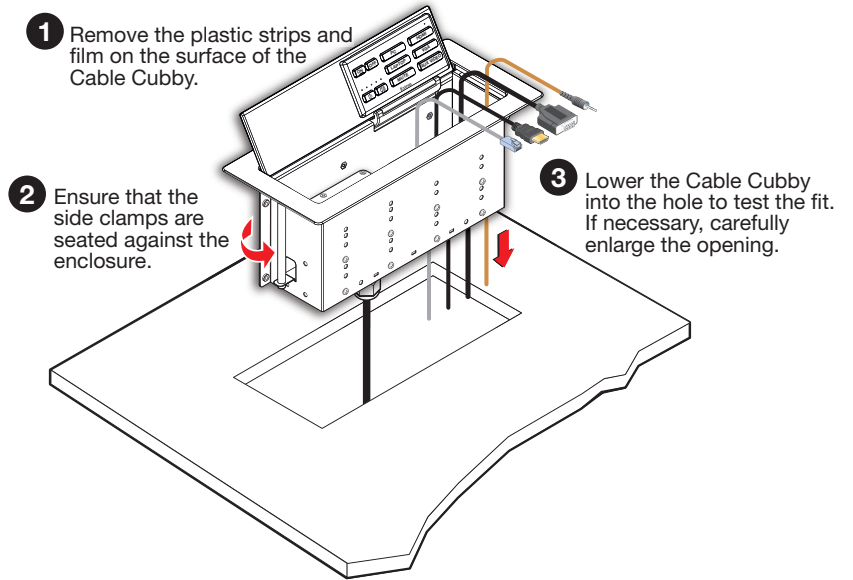
Figure 7. Insert EBP 1200C Enclosure into the Table
