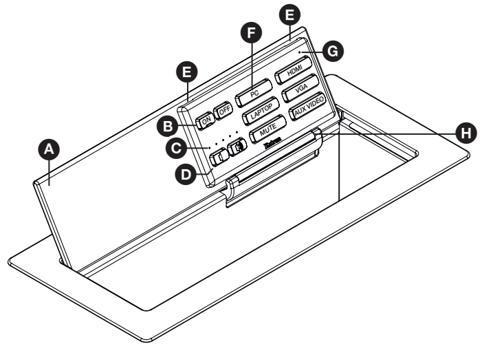
Figure 11. EBP 1200C Front Panel
