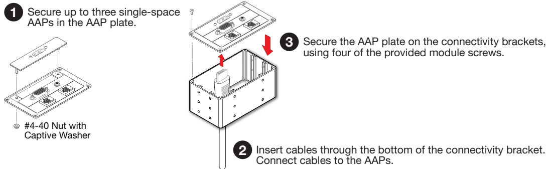
Figure 3. Assembling the AAP Module
