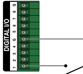
Figure 2. Digital Input — Dry Contact
