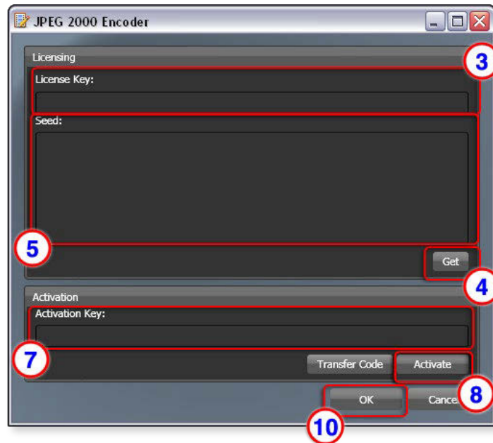
Figure 4. Licensing and Activation Screen
