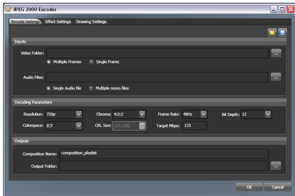
Figure 5. Encode Settings Tab
