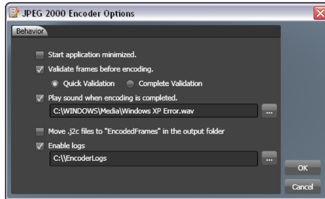
Figure 16. JPEG 2000 Encoder Options Screen
