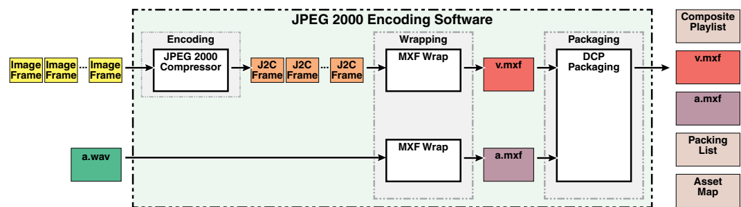
Figure 19. Encoding, Wrapping, and Packaging Process
