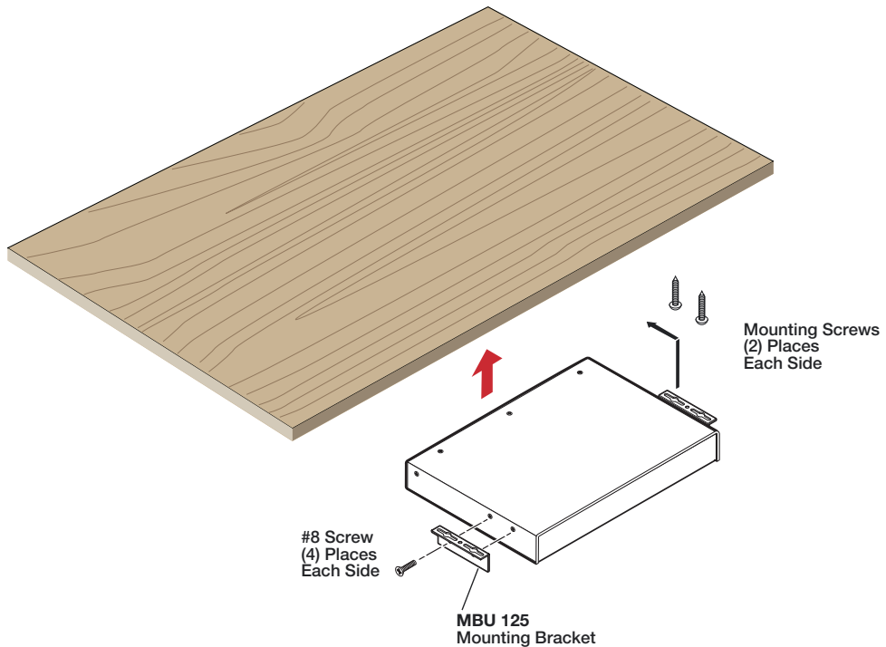
Figure 62. Under-Desk Mounting
