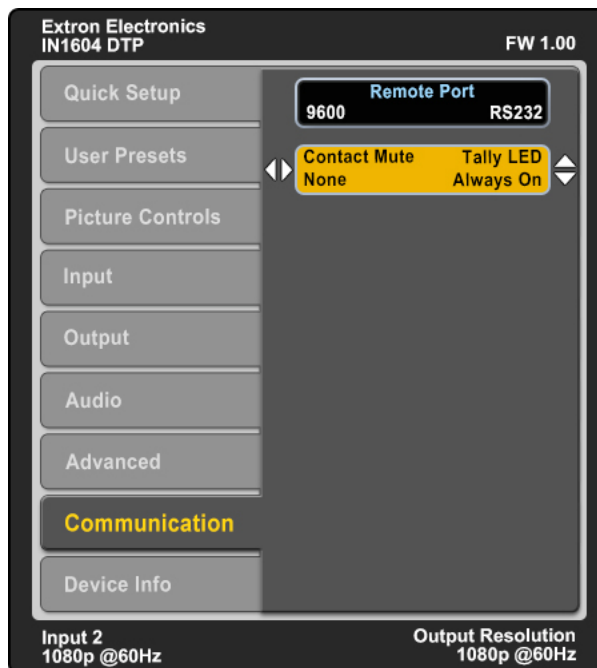
Figure 19. Communication Submenu
