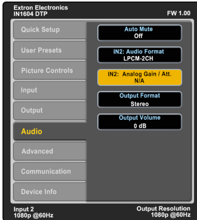
Figure 16. Audio Submenu
