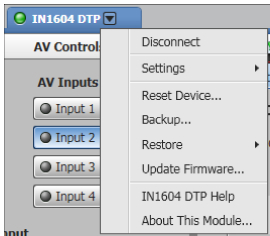
Figure 33. Device Menu
