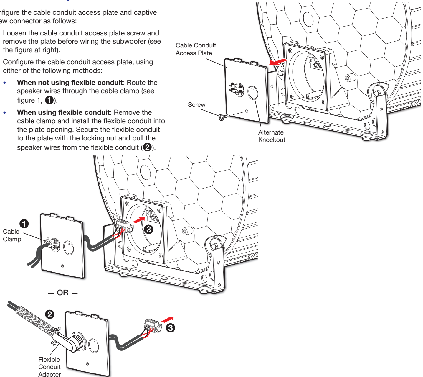
Figure 1. Connection Using a Cable Clamp or Flexible Conduit
