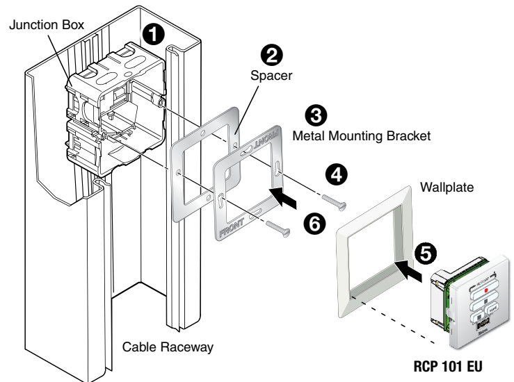
Figure 7. Mounting in a Cable Raceway
