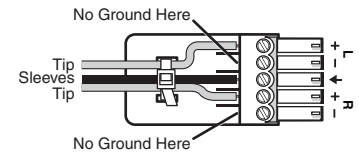
Unbalanced Audio Output
