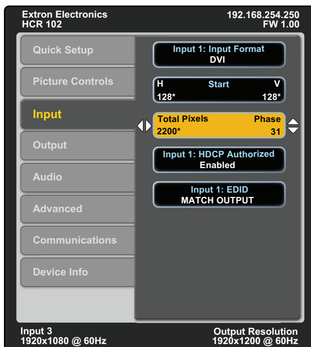
Figure 28. Input Submenu
