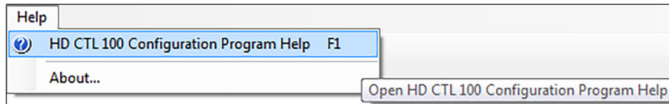
Figure 4. Help Menu
