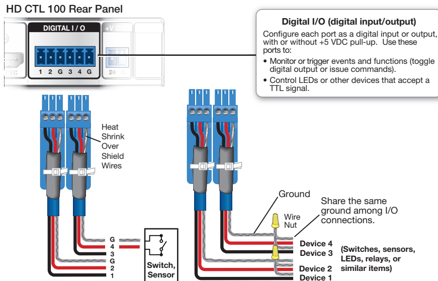
Figure 3. Wiring the Digital I/O Connectors
