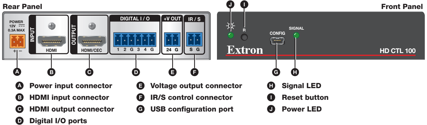
Figure 1. HD CTL 100 Rear and Front Panels
