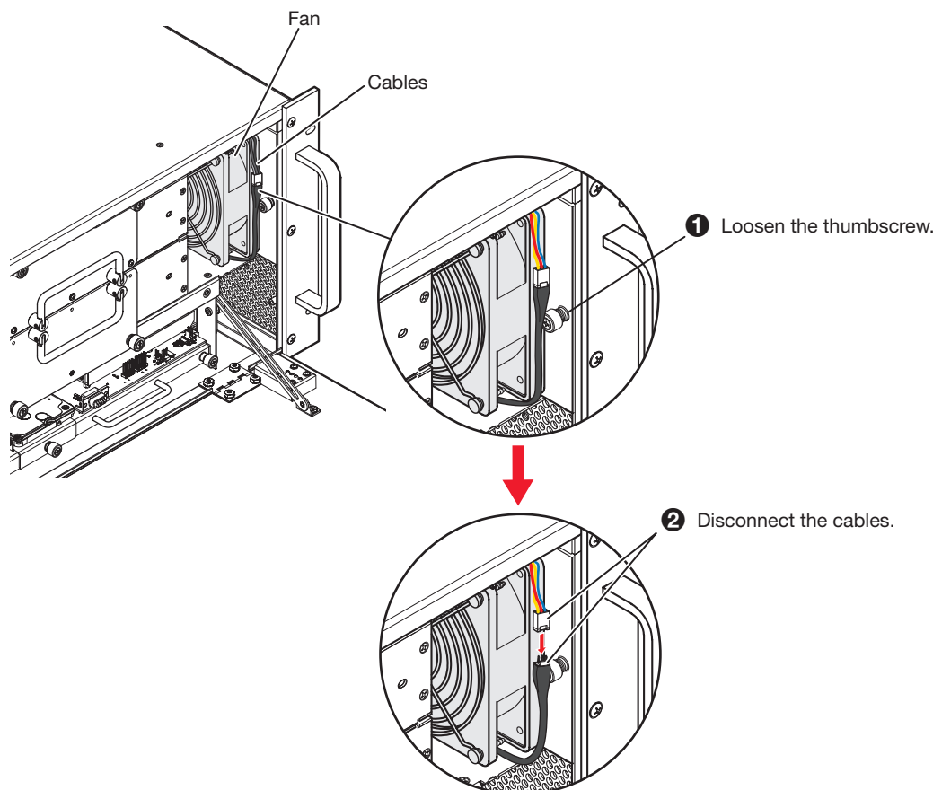
Figure 2. Detaching the Top Fan
