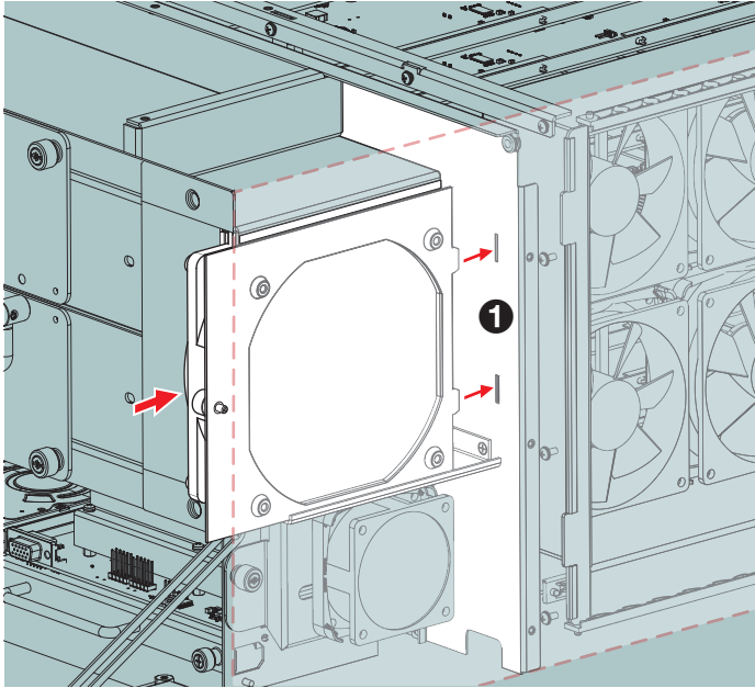
Figure 5. Inserting the Replacement Fan
