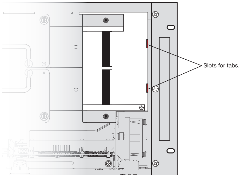
Figure 4. Slots for Tabs in the Back of the Fan Compartment
