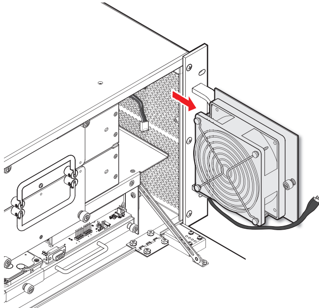
Figure 3. Sliding the Power Supply Fan Out of the Chassis
