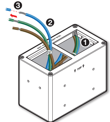
Figure 1. AC 102 Module with Wires
