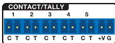
Figure 7. CONTACT/TALLY Ports
