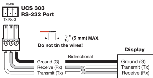
Figure 6. Wiring for RS-232 Display Control
