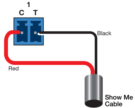
Figure 8. Show Me Cable Connecting Contact and Tally Ports
