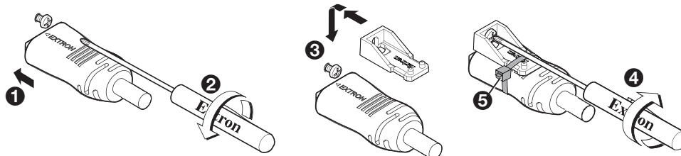
Figure 9. LockIt Plus Installation Diagram
