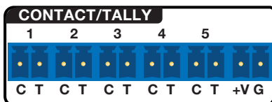
Figure 6. CONTACT/TALLY Ports
