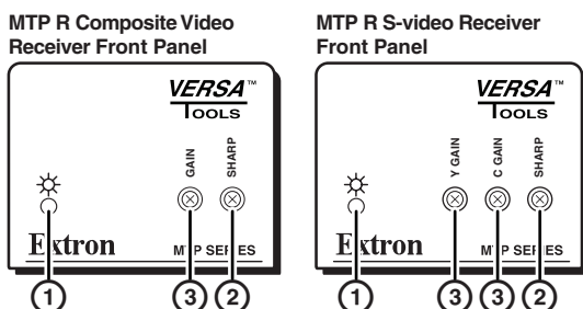
Figure 2-1 — MTP receiver front panels
