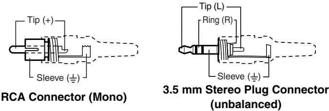
Figure 1-3 — Typical audio connectors
