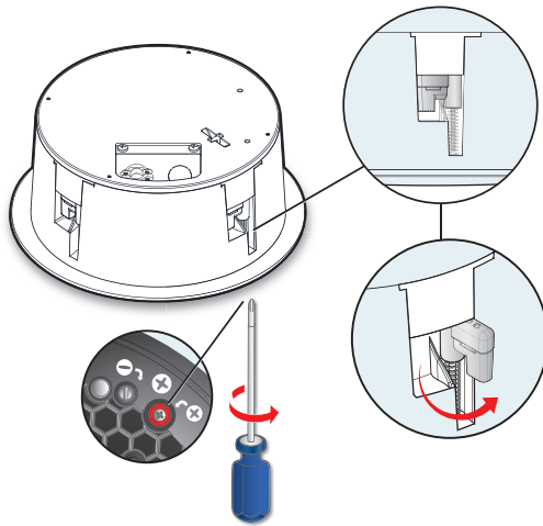
Figure 3. Accessing the Locking Arm Insert
