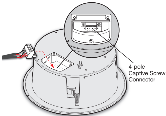
Figure 6. Secure Cabling via Cable Clamp
