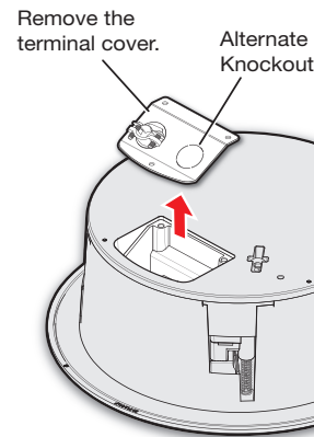
Figure 5. Removing the Cable/Conduit Access Plate
