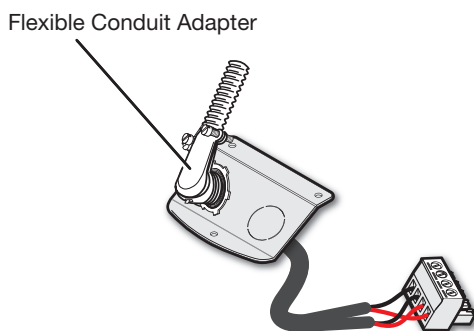
Figure 7. Secure Cabling via Conduit Adapter
