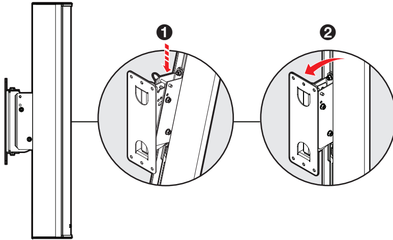
Figure 16. Attaching Speaker to Wall Mount
