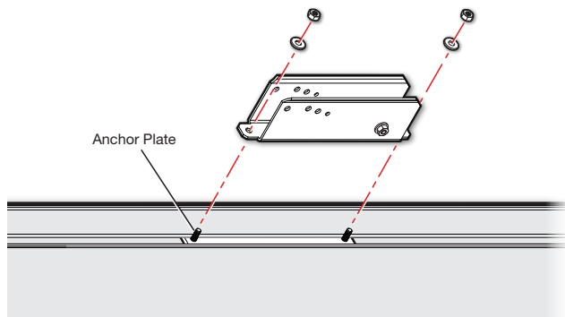
Figure 13. Securing Speaker Bracket to Anchor Plate
