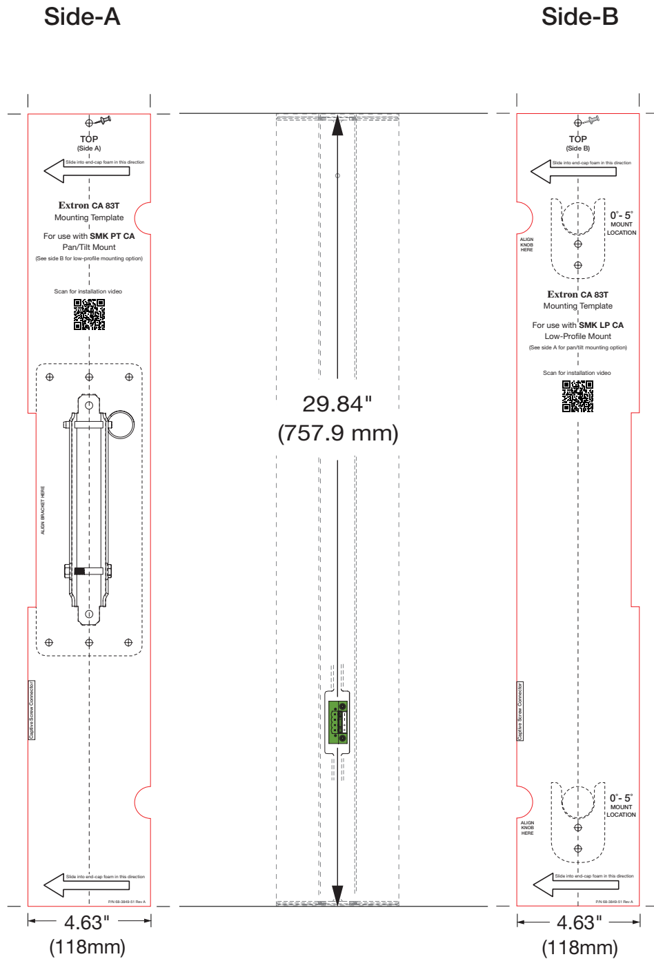
Figure 21. CA 83T Speaker Mounting Template (NOT to scale)
