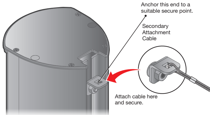
Figure 19. Securing the Secondary Tie-off
