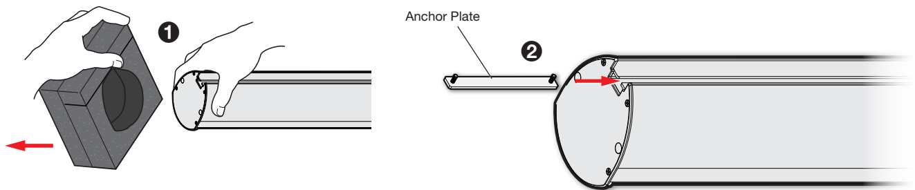
Figure 12. Sliding Anchor Plate into T-slot
