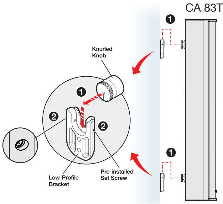
Figure 9. Securing the CA Speaker Low Profile Mount
