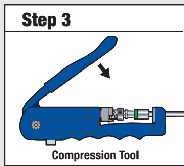
Compress connector and cable together.
