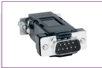
VGAF-9DM VGA female to 9-pin D male adapter Part # 26-170-03
