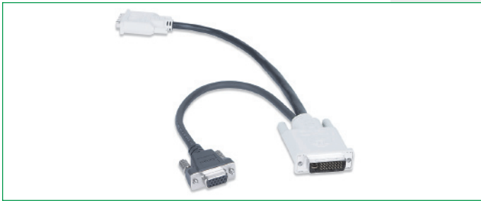
DVIIM-VGAF/DVIIF DVI-I Male to 15-pin HD Female and DVI-D Female "Y" Adapter 12" (30 cm) Part # 26-612-01
