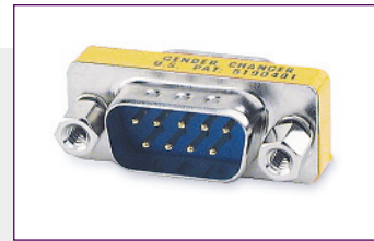
9D GCM 9-pin D male-male gender changer Part # 10-438-01
