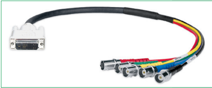
SY DVIA-RGBHVF DVI-A Male to 5 BNC Female 6" (15 cm) Part # 26-609-01
