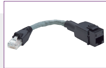
NETXA M-F Ethernet crossover adapter to connect a computer directly to an IP Link® product Part # 26-615-01
