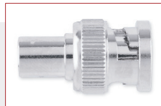
T-BNC 75 ohm, BNC male termination adapter Part # 100-234-01 (Qty. 10) Part # 100-234-03 (Qty. 50) Part # 100-234-04 (Qty. 100)
