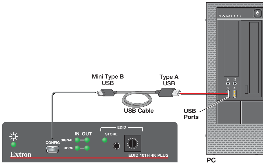
Figure 14. Connecting a PC to the Front Panel USB Port
