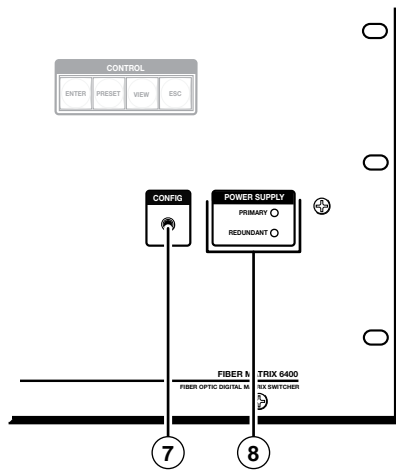
Figure 2-7 — Front panel configuration port
