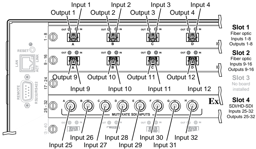
Figure 2-1 — Arrangement of inputs and outputs on the I/O boards
