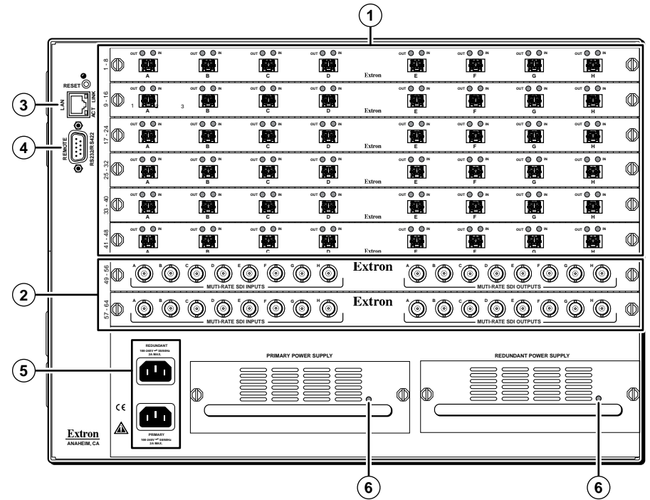
Figure 2-2 — Fiber Matrix 6400 Switcher rear panel
