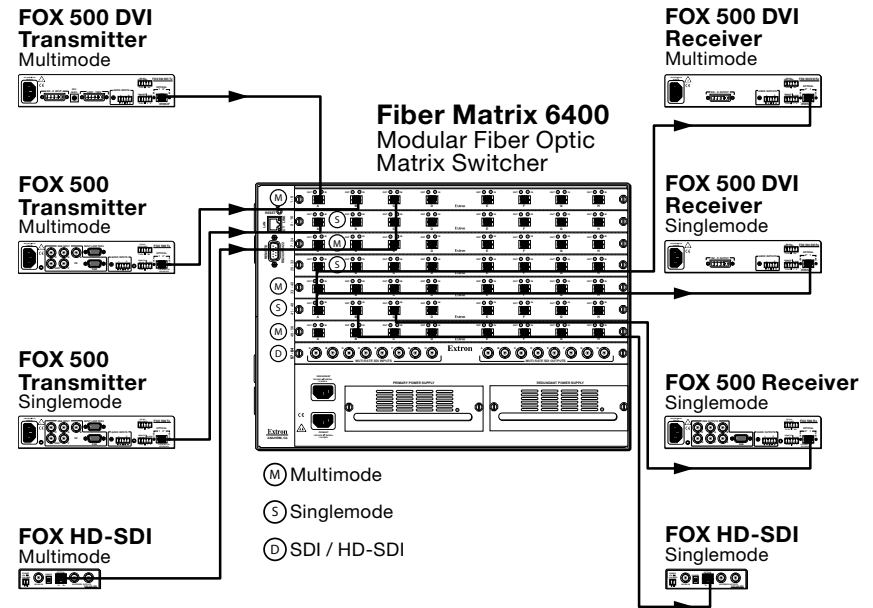
Figure 1-1 — Typical Fiber Matrix 6400 application
