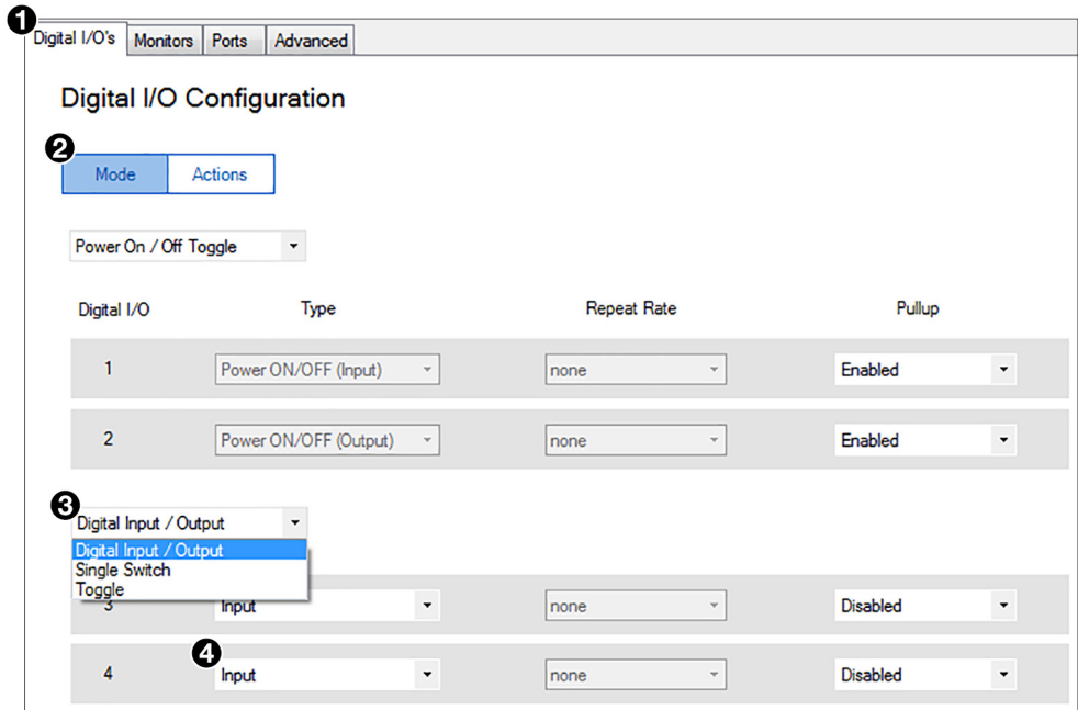
Figure 32. Configuring Digital I/O Port 4 as an Input for the Occupancy Sensor
