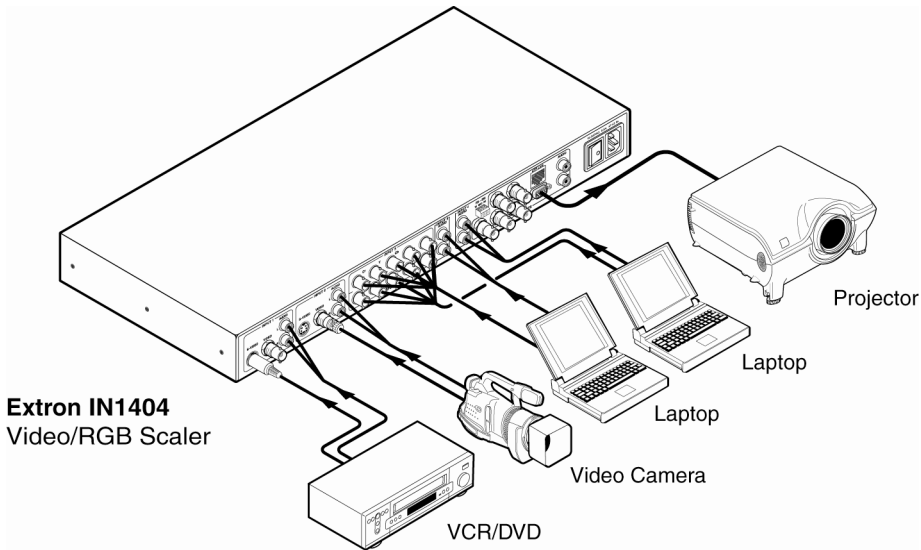
Figure 1. — IN1404 application diagram
