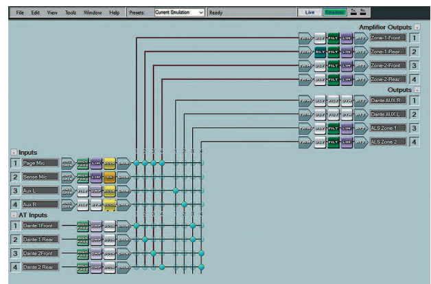
Extron DSP Configurator-Software
