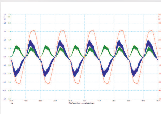
FIG. 15: Course of mains voltage (red), mains current (blue) and the power consumption (green) calculated from them with an RMS value of 253 VA. The power factor is 0.94 and the \cos \phi value is 0.96.
