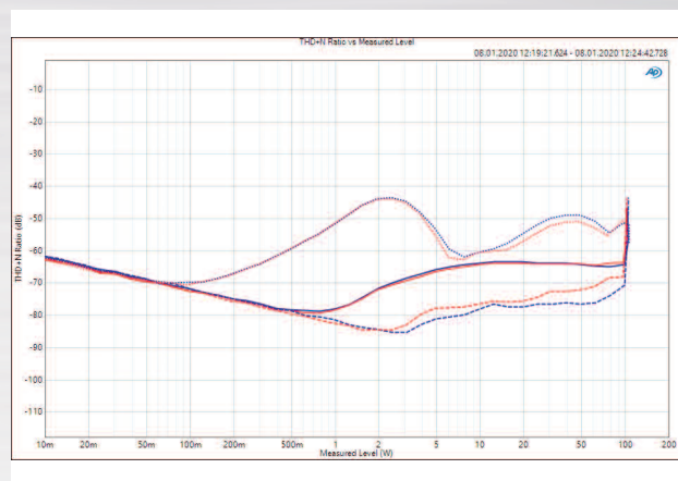
FIG. 06: Distortion values (THD+N) for channel 1 (bl) and 2 (rt) as a function of power (x-axis) for a load of 2x 8 Ω measured at 100 Hz (dashed), at 1 kHz (solid) and 6.3 kHz (dotted).
