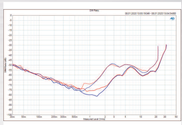
FIG. 10: Transient intermodulation distortions (DIM) for channel 1 (bl) and 2 (rt) depending on the output voltage [x-axis] for a load of 2 \times 4 \Omega [solid lines] and 2 \times 8 \Omega [dashed lines].
