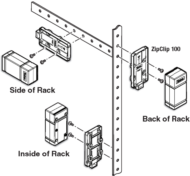
Figure 3. Rack Rail Mounting
