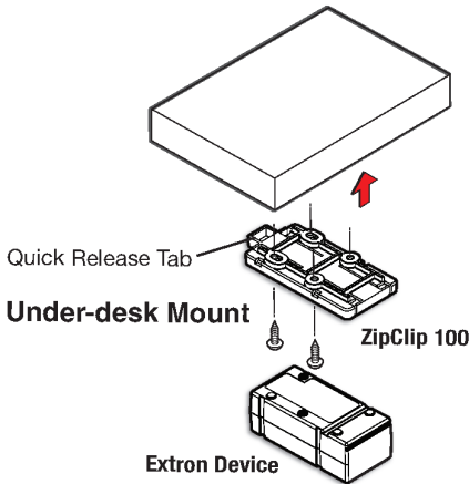
Figure 2. Under-desk Mounting
