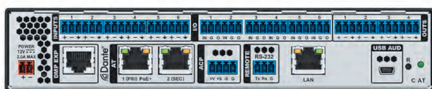
DMP 64 Plus C AT - 后面板
