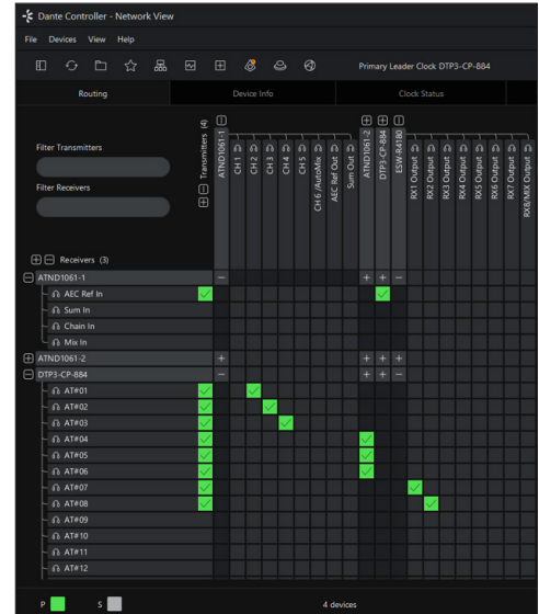
Figure 18. Subscriptions
