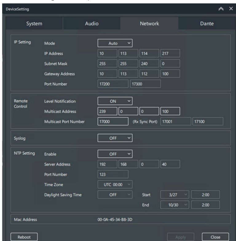
Figure 17. DeviceSetting Window
