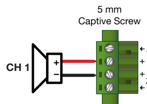
Figure 3. Captive Screw Audio Cable Wiring
