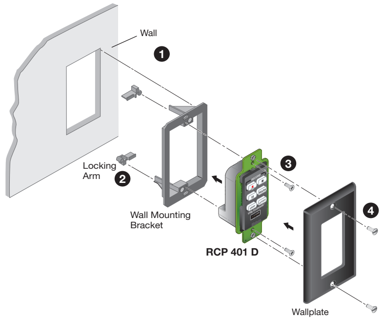
Figure 4. Mounting with a Wall Mounting Bracket
