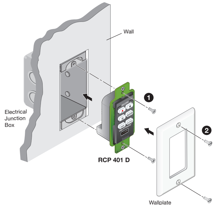
Figure 5. Mounting with an Electrical Junction Box
