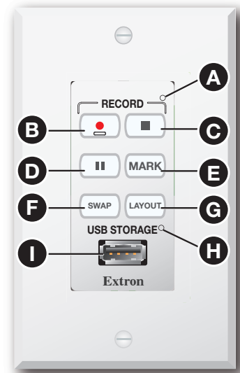
Figure 1. RCP 401 D Front Panel
